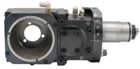
Thread Whirling Head
