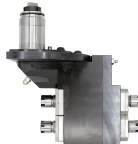
Double Angular Drilling Head
